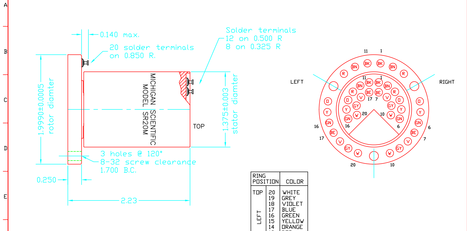
SR20M slip ring assembly
